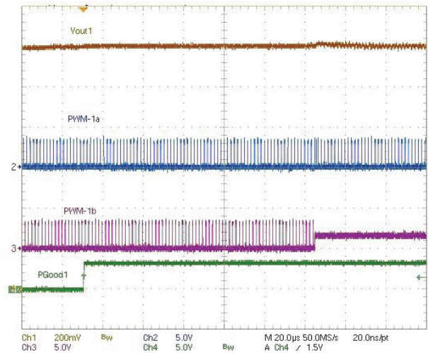
Figure 28: Phase Shed 2Φ à 1Φ at startup
