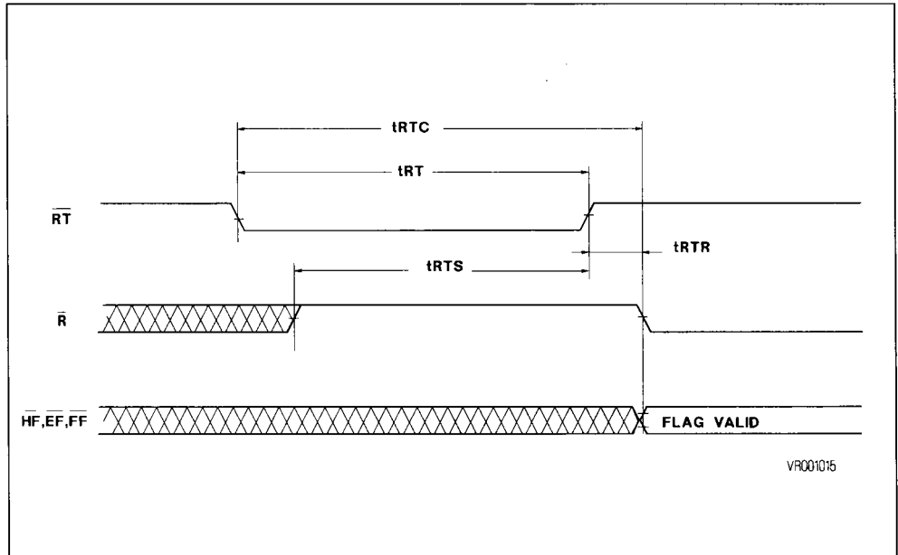
Figure 8. Retransmit Waveforms
