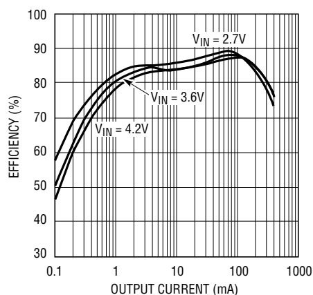
Single Li-Ion to 1V/200mA Regulator Using All Ceramic Capacitors Optimized for Small Footprint
