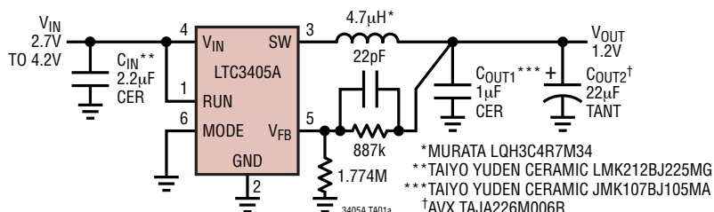
Single Li-Ion to 1.2V/300mA Regulator Using Ceramic and Tantalum Output Capacitors
