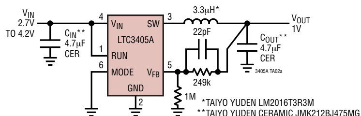
Single Li-Ion to 1V/200mA Regulator Using All Ceramic Capacitors Optimized for Small Footprint
