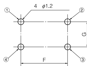
Recommended PWB piercing plan
