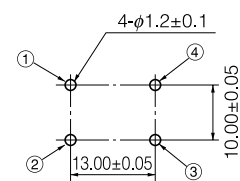
Recommended PWB piercing plan
