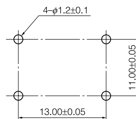
Recommended PWB piercing plan
