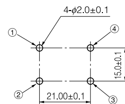
Recommended PWB piercing plan
