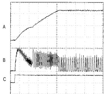
POWER-UP RESPONSE
