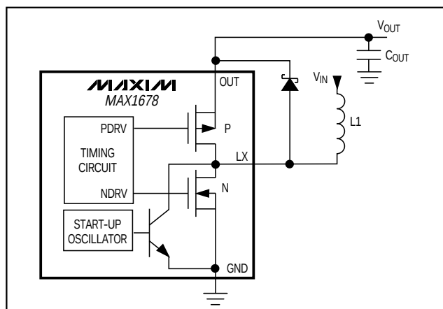
Figure 3. External Schottky Diode to Improve Start-Up with Heavy Load
