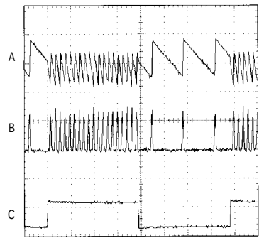
LOAD-TRANSIENT RESPONSE
