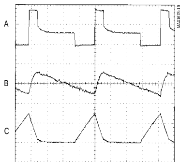
SWITCHING WAVEFORM
