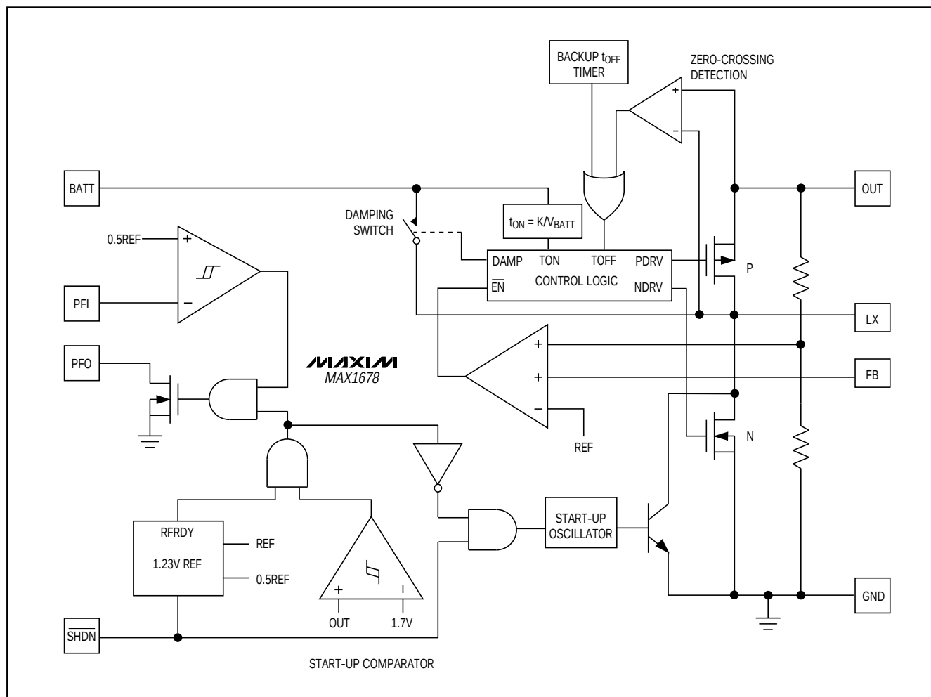
Figure 1. Functional Diagram
