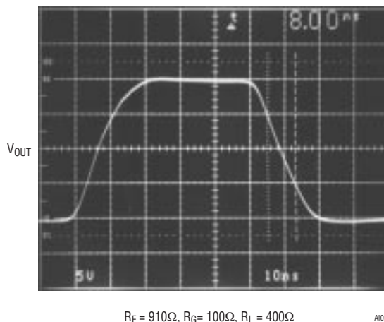
Large-Signal Transient Response, A_V = +10
