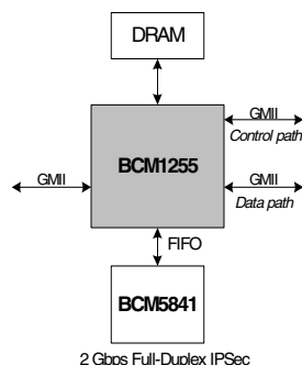
VPN/Firewall Application
