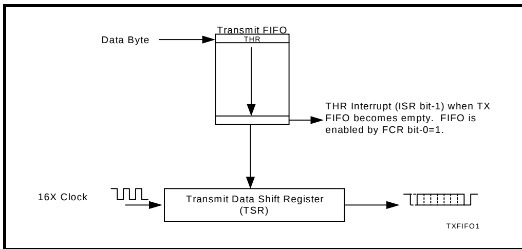
FIGURE 8. TRANSMITTER OPERATION IN FIFO MODE
