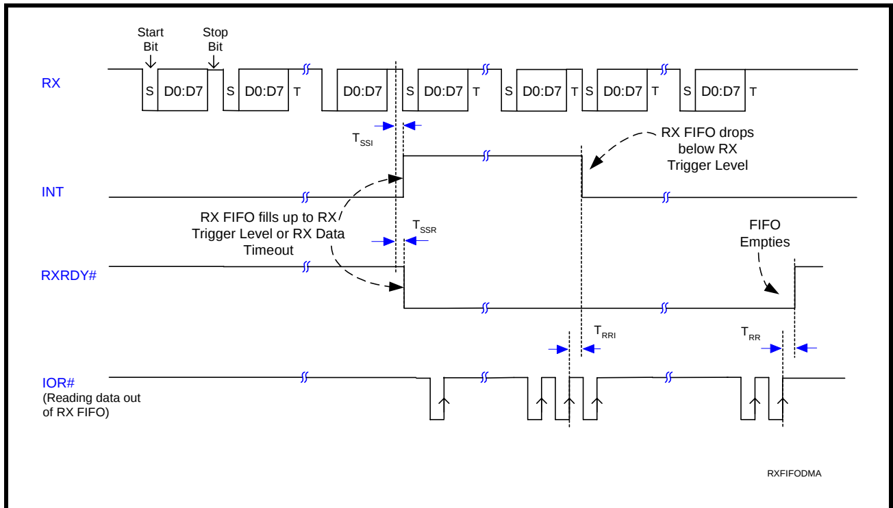
FIGURE 19. RECEIVE READY & INTERRUPT TIMING [FIFO MODE, DMA ENABLED] FOR CHANNELS A & B
