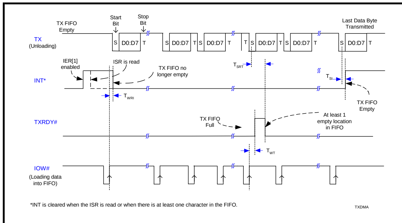
FIGURE 21. TRANSMIT READY & INTERRUPT TIMING [FIFO MODE, DMA MODE ENABLED] FOR CHANNELS A & B
