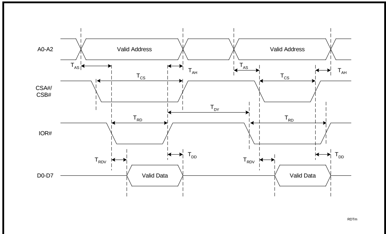
FIGURE 14. DATA BUS READ TIMING
