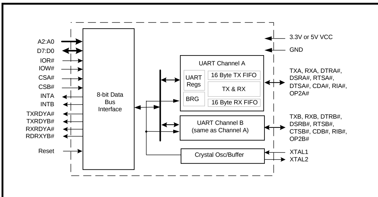
FIGURE 1. ST16C2550 BLOCK DIAGRAM
