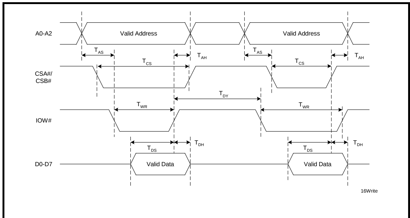
FIGURE 15. DATA BUS WRITE TIMING
