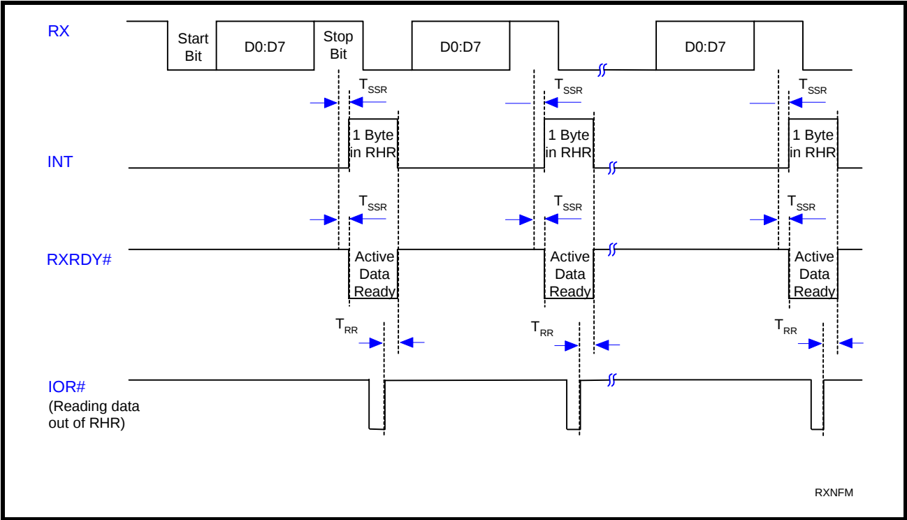
FIGURE 16. RECEIVE READY & INTERRUPT TIMING [Non-FIFO Mode] FOR CHANNELS A & B
