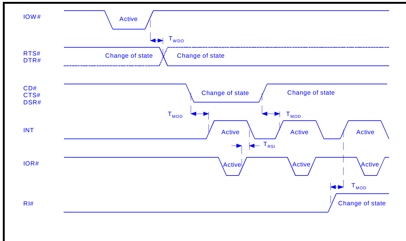
FIGURE 13. MODEM INPUT/OUTPUT TIMING FOR CHANNELS A & B
