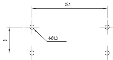
PIERCING PLAN
