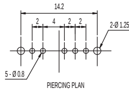
PIERCING PLAN
