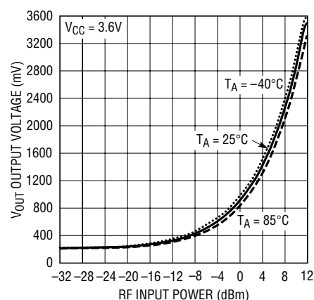
Typical Detector Characteristics, 6000MHz, Gain = 2, V OS = 0V
