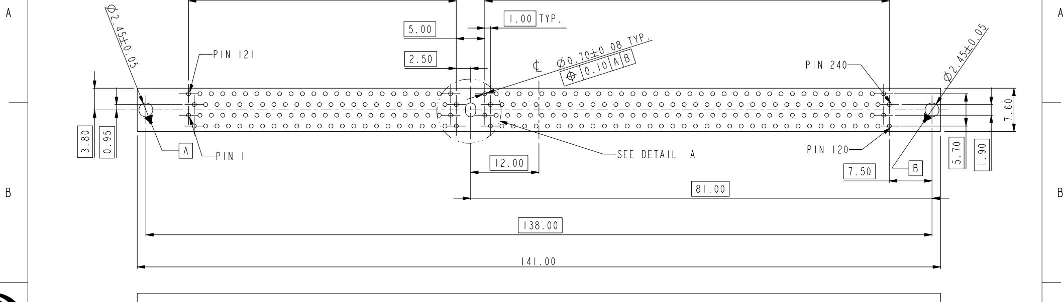
RECOMMENDED CIRCUIT BOARD HOLE LAYOUT
