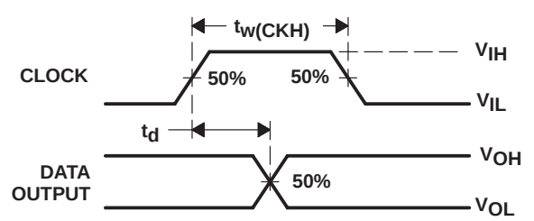
Figure 4. Data Output Switching Times
