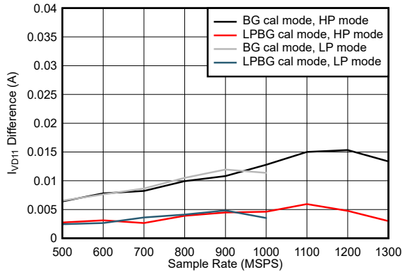
Figure 5-121. Dual Channel, I_{VD11} Change with Calibration Mode
