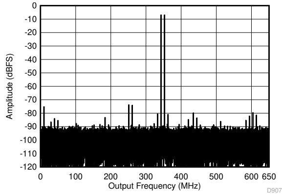
Figure 5-49. Two Tone FFT at 348 MHz Center
