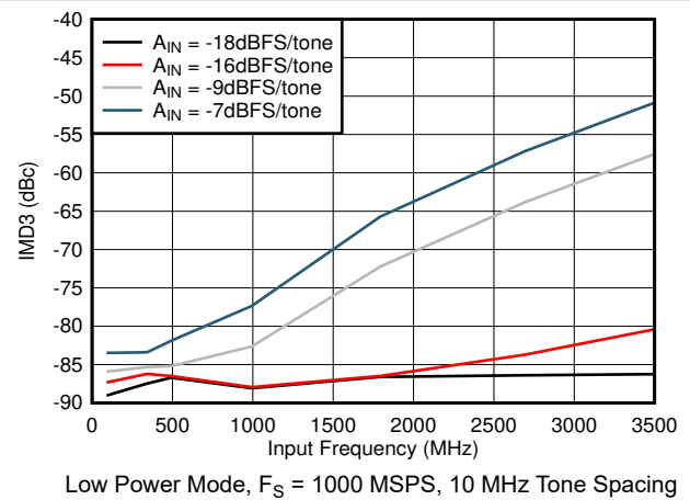
Figure 5-58. IMD3 vs Input Frequency
