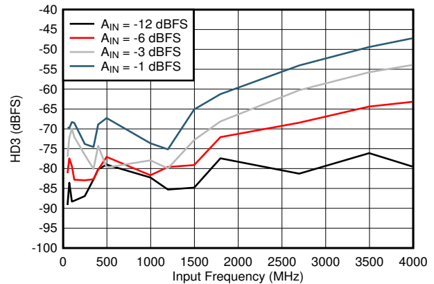
Figure 5-20. HD3 vs Input Frequency
