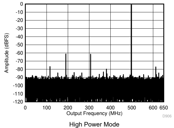
Figure 5-8. Single Tone FFT at 1797 MHz and -1 dBFS
