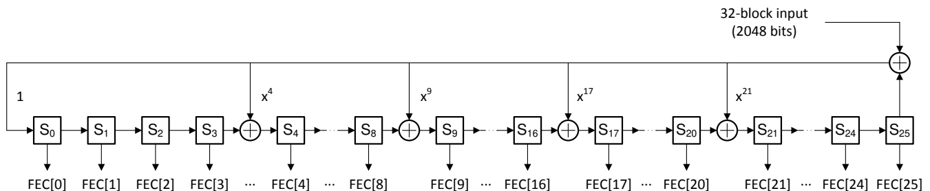
Figure 6-10. FEC Parity Bit Generator
