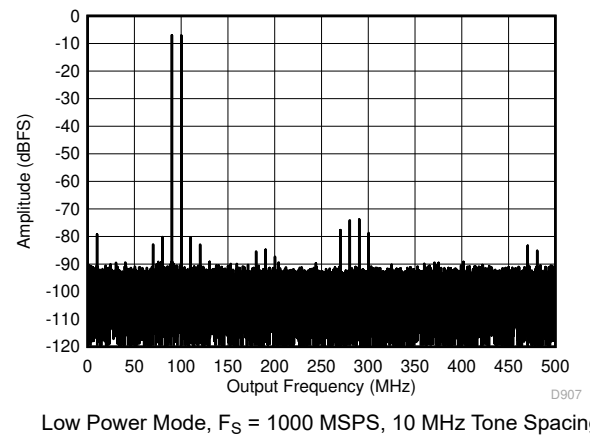
Figure 5-54. Two Tone FFT at 95.07 MHz Center
