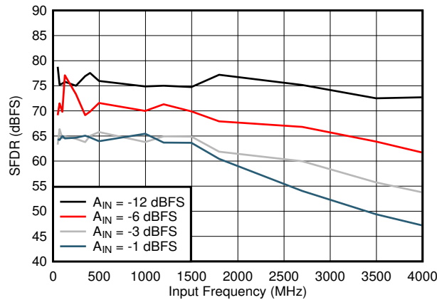
Figure 5-15. SFDR vs Input Frequency
