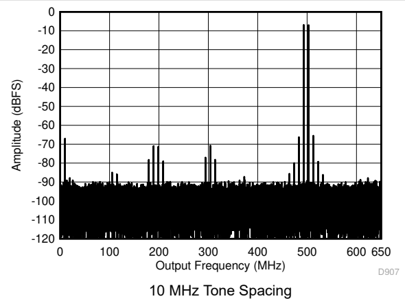
Figure 5-52. Two Tone FFT at 1798 MHz Center
