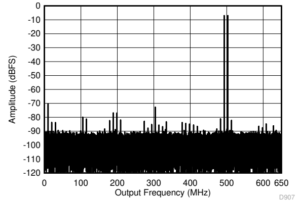
Figure 5-50. Two Tone FFT at 498 MHz Center
