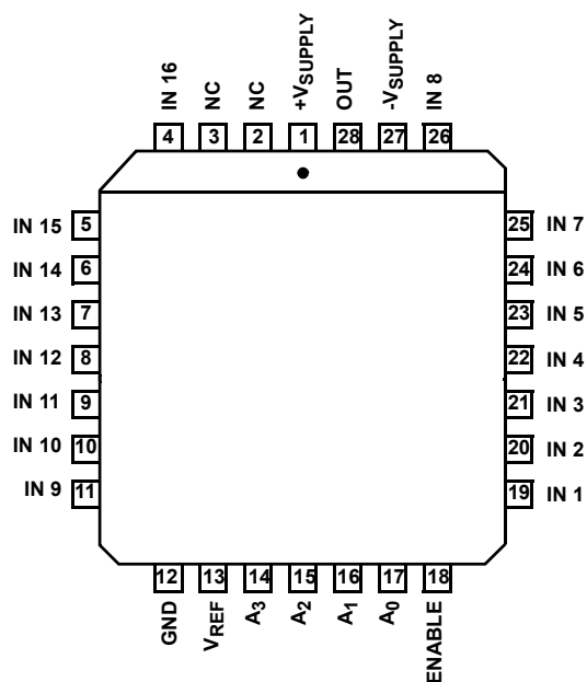
HI-546/883 (28 LD CLCC) TOP VIEW
