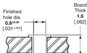
Solder Post
