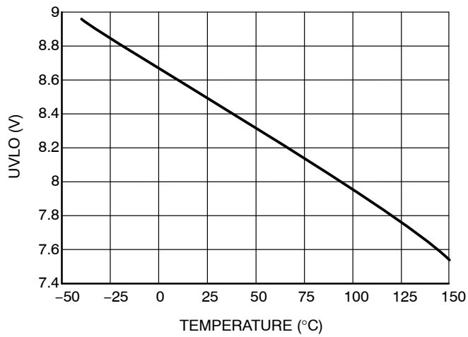
Figure 6. UVLO Turn-On
