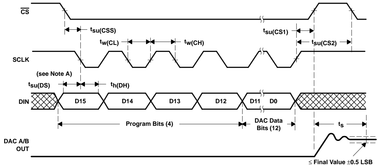
Figure 1. Timing Diagram for the TLC5618A
