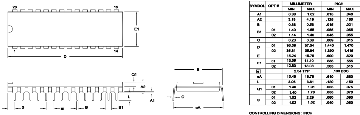
Figure 63 displays the 28-pin PDIP package available for Z8 Encore! XP F0822 Series devices.
