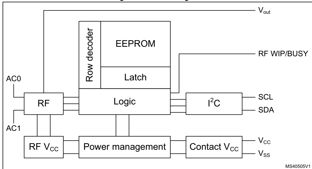
Figure 5. Circuit diagram
