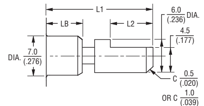
FLATTED SHAFT
