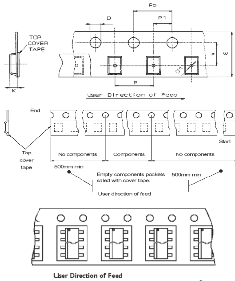
Figure 21. PowerSSO24, tape drawings
