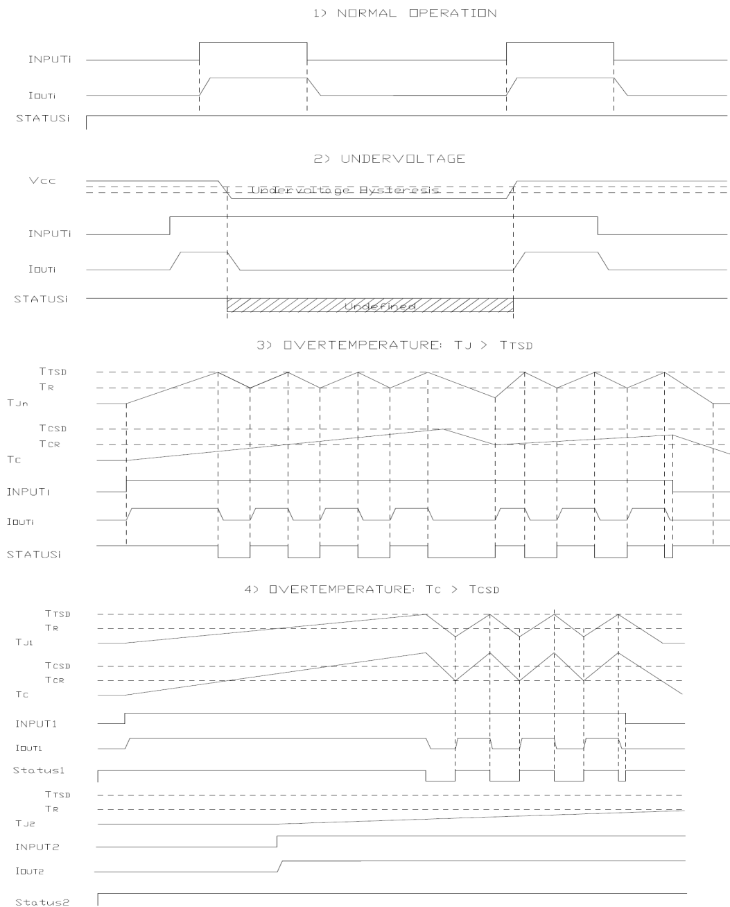
Figure 7. Switching waveforms
