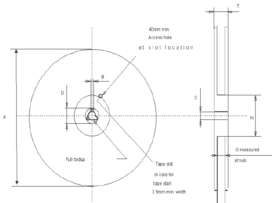
Figure 20. PowerSSO24, reel shipment
