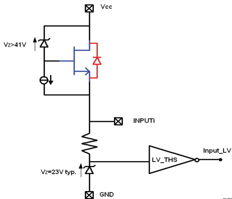
Figure 8. Input circuit
