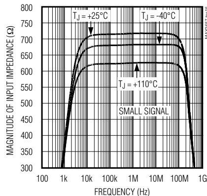
INPUT IMPEDANCE vs. FREQUENCY
