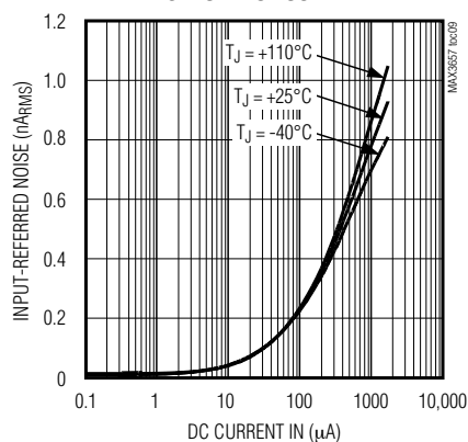
INPUT-REFERRED RMS NOISE vs. DC INPUT CURRENT
