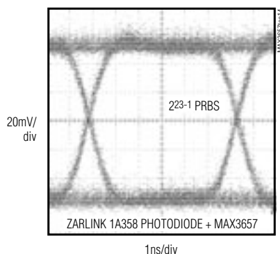
OUTPUT EYE DIAGRAM (-1dBm OPTICAL INPUT)
