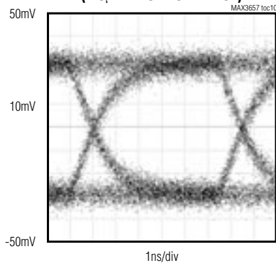
OUTPUT EYE DIAGRAM (1.0 \mu A ELECTRICAL INPUT)
