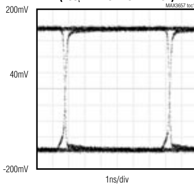
OUTPUT EYE DIAGRAM (100 \mu A ELECTRICAL INPUT)
