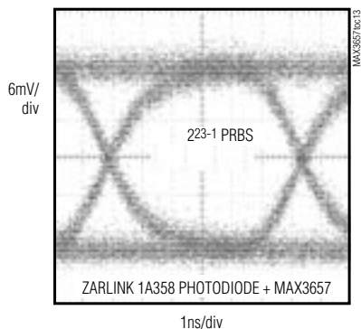
OUTPUT EYE DIAGRAM (-30dBm OPTICAL INPUT)
