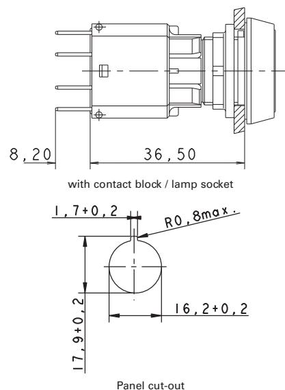
Panel cut-out
