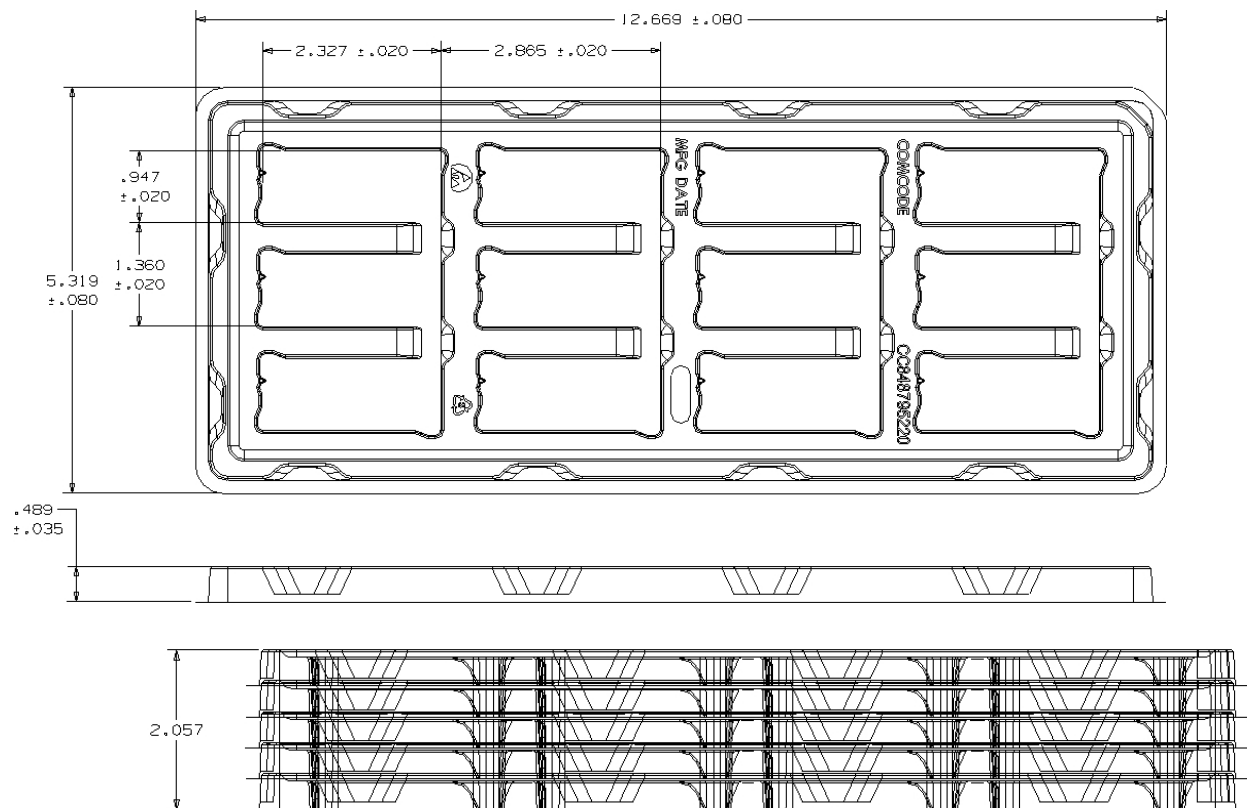
Figure 27. Surface Mount Packaging Tray
