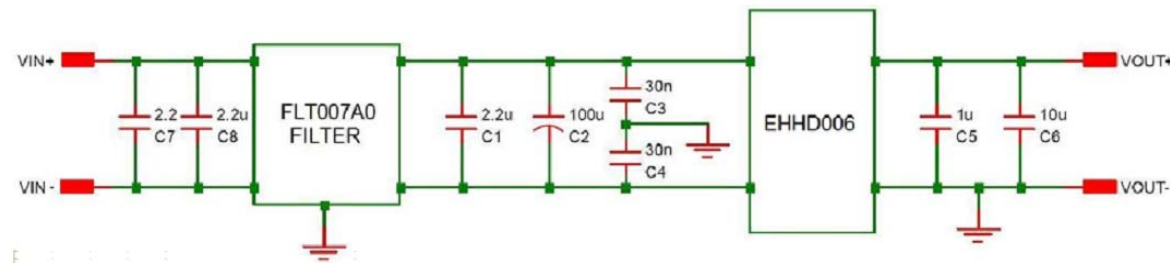
Figure 26. EMC Considerations
