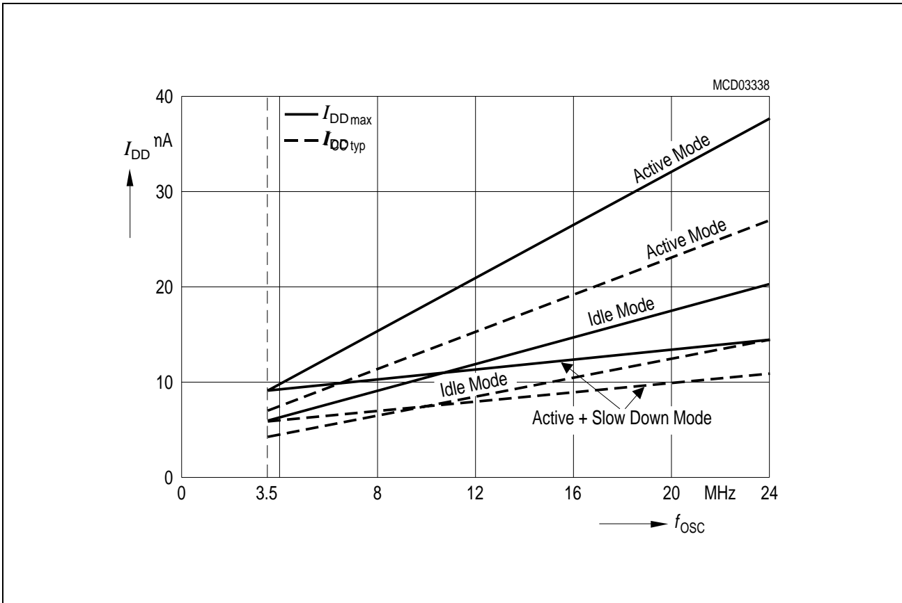
Figure 26 IDD Diagram
