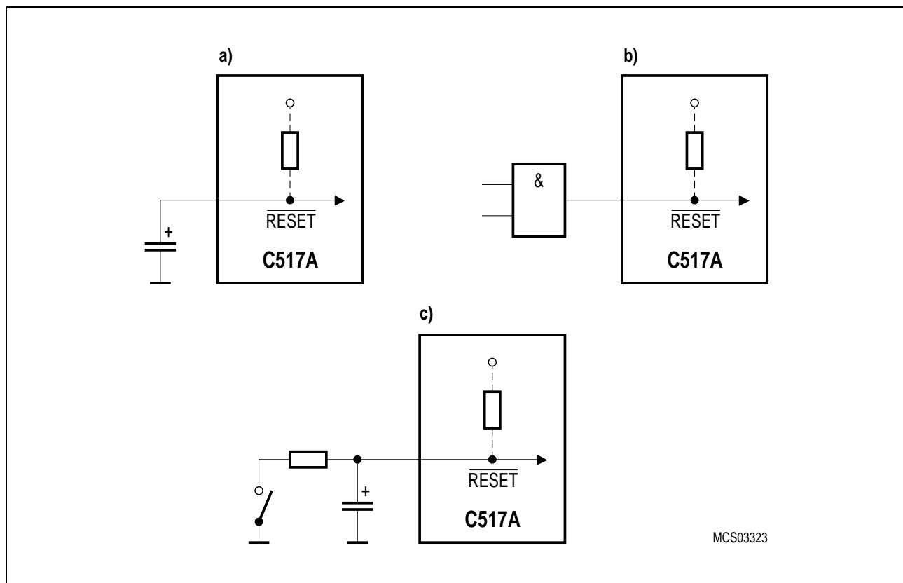
Figure 7 Reset Circuitries
