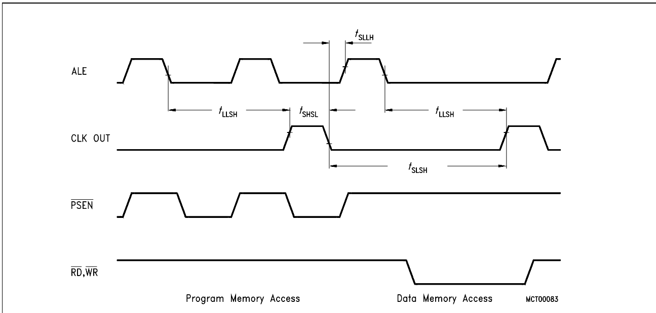
Figure 29 CLKOUT Timing
