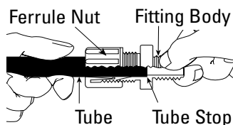
*50 P.S.I. Ferrule nut with integral sleeve low pressure application soft plastic tubing
