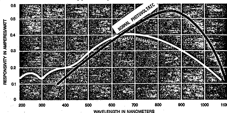
Typical Spectral Response.
