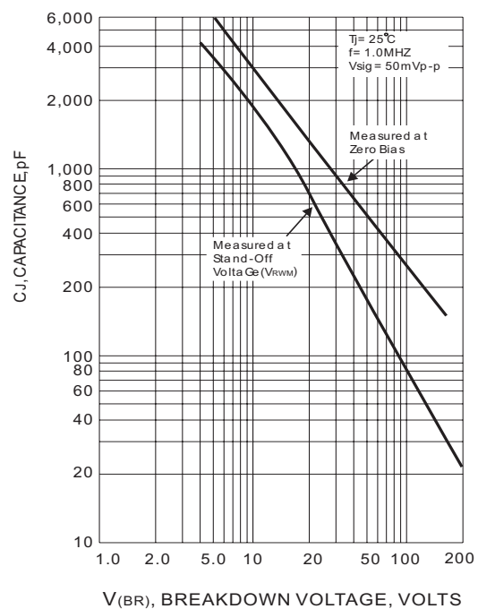
Fig.4 TYPICAL CAPACITANCE
