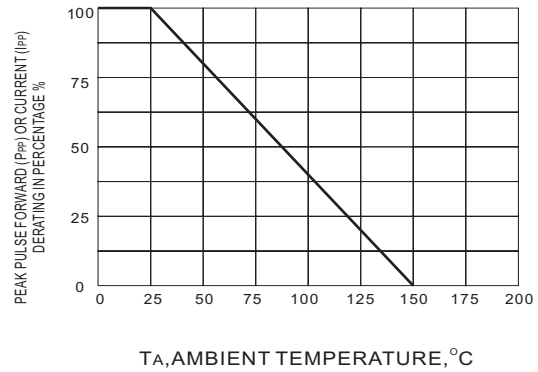
Fig.2 DERATING CURVE
