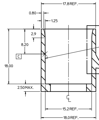
SECTION Z-Z
