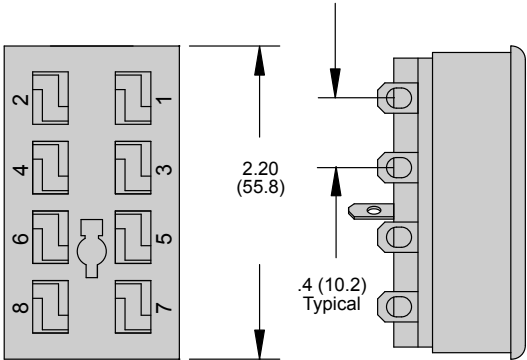
8 Pin Socket
