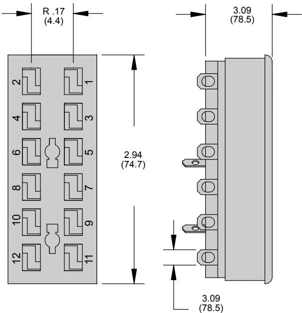
12 Pin Socket
