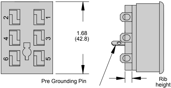
6 Pin Socket
