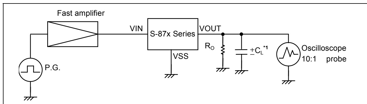
Figure 26 Rectangular wave from 0 V to 10 V (Type 2)
