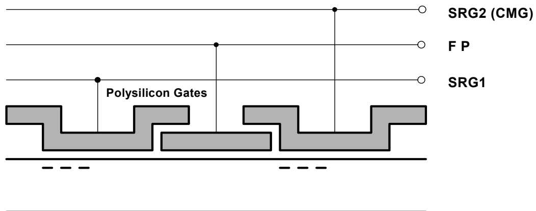
Pixel Cross Section
