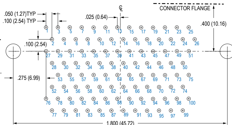
100 PIN M83513/12-H
