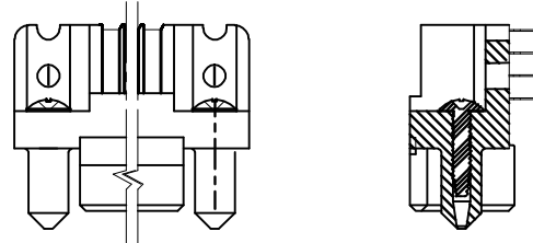
SECTION U-U
