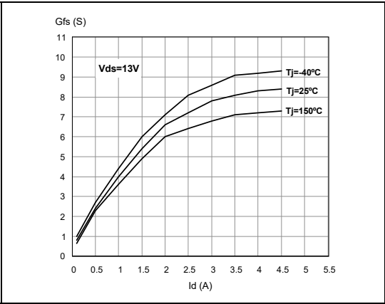
Figure 12. Transconductance
