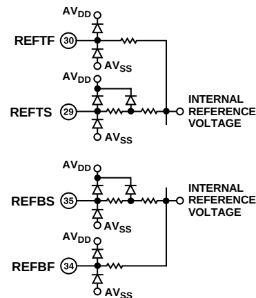
Figure 2. Equivalent Circuits
