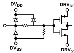
b) Three-State, Standby
