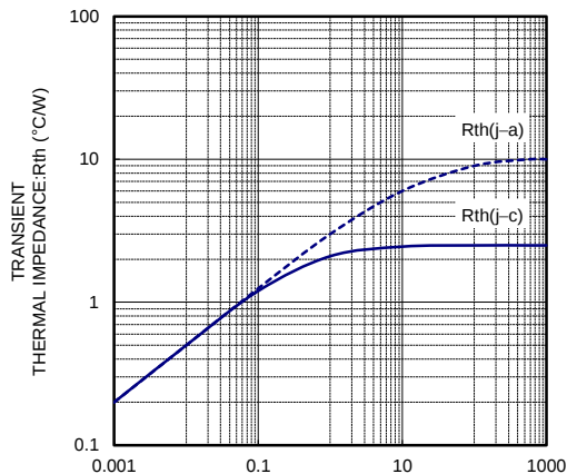
R_th-t CHARACTERISTICS
