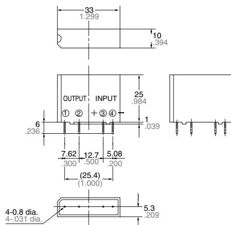
External dimensions
