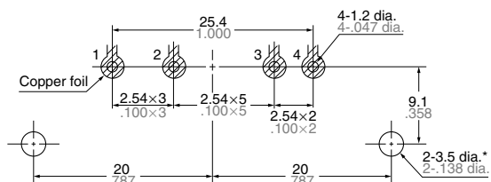
Mounting hole location (Copper-side view)
