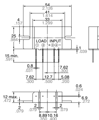
External dimensions
