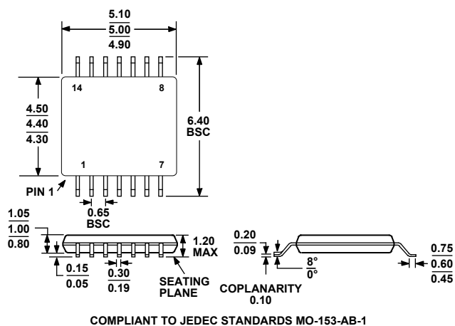
Figure 55. 14-Lead Thin Shrink Small Outline Package [TSSOP] (RU-14)
