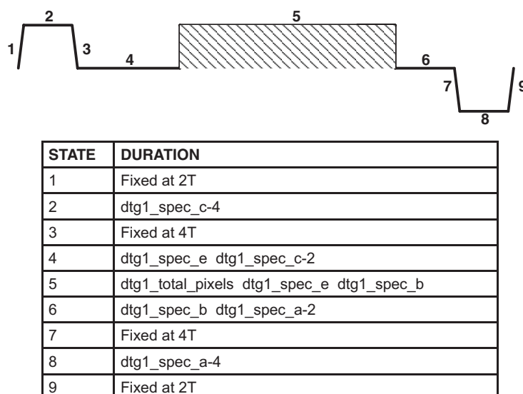
Figure 4-18. HDTV Line Type ACTIVE_VIDEO
