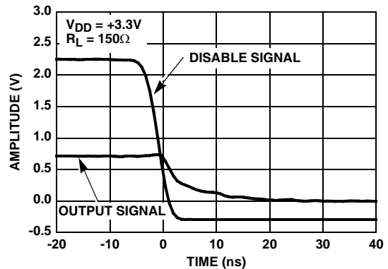
FIGURE 14. DISABLE TIME
