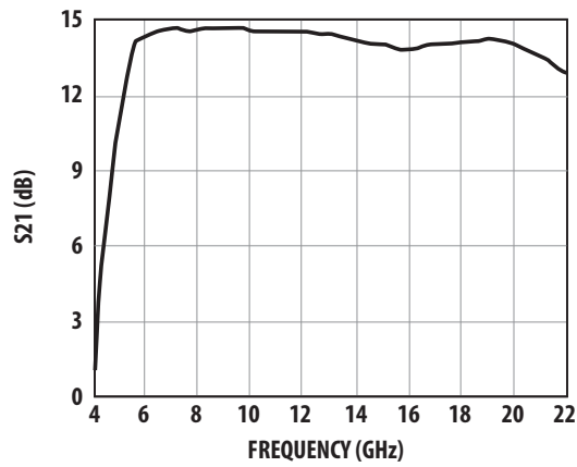
Figure 1. Gain.
