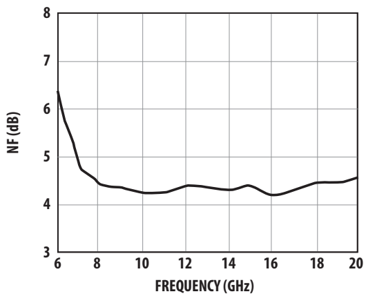
Figure 5. Noise Figure.
