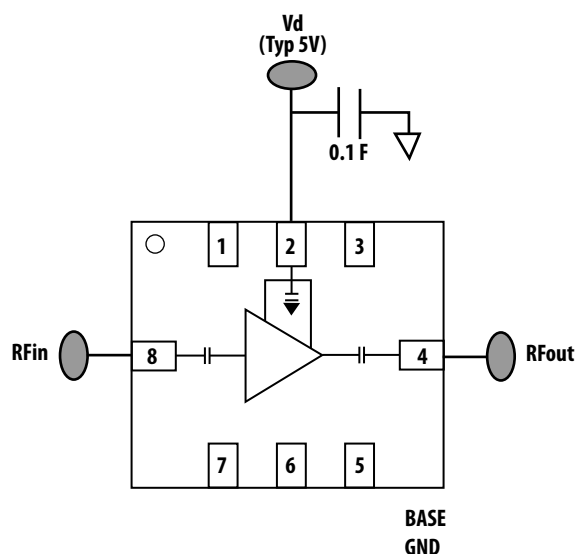
Figure 19. Typical Application.
