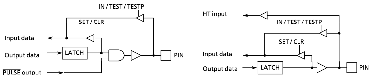
Figure 2-1. port R4
