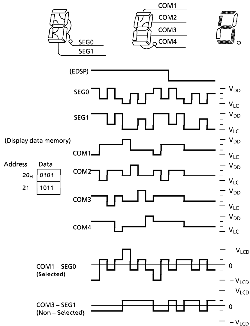
Figure 2-13. 1/4 Duty (1/3 Bias) Drive
