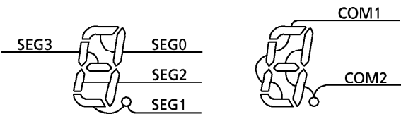
Figure 2-14 Example of the COM, and SEG Pin Connection.
