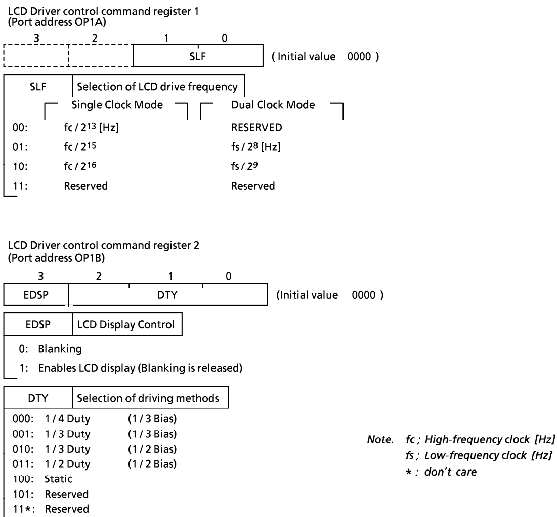
Figure 2-9. LCD Driver control Command Register
