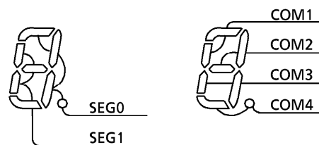
Figure2-13. Example of the COM, and SEG Pin Connection
