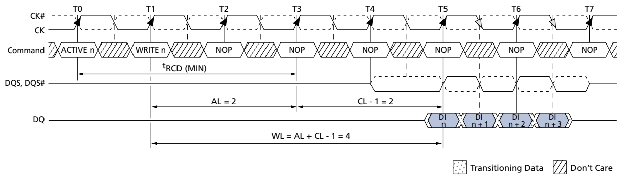
Figure 39: WRITE Latency
