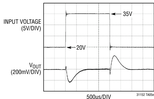
Fast (20μs) Input Voltage Transient, V_{IN} = 20V to 35V
