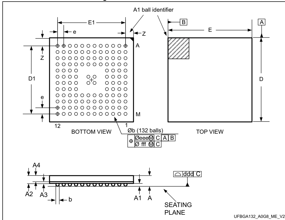
Figure 40. UFBGA132 outline
