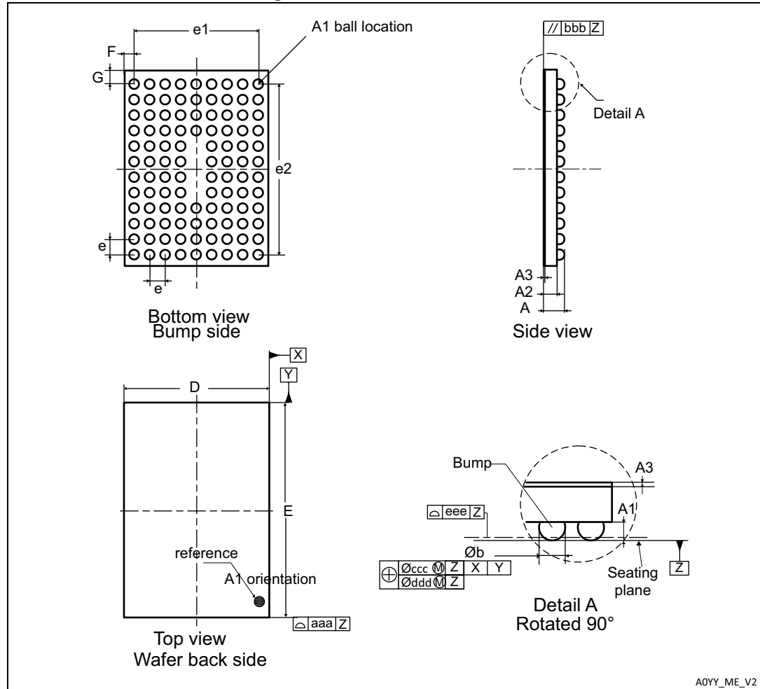
Figure 37. WLCSP104 outline
