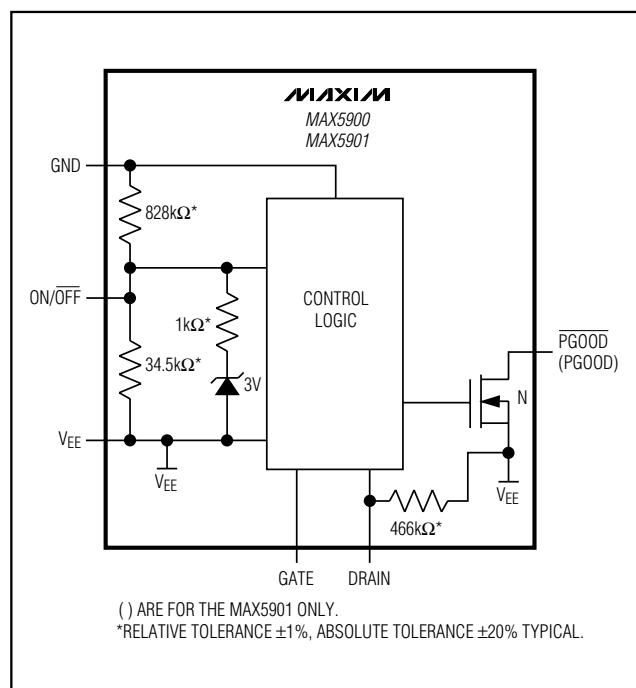
Figure 1. Functional Diagram
