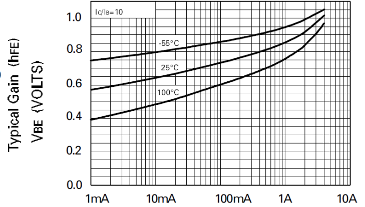
Collector Current
