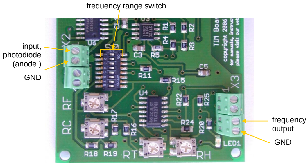
Fig. 3: Current-to-Frequency Converter input, output and switches
