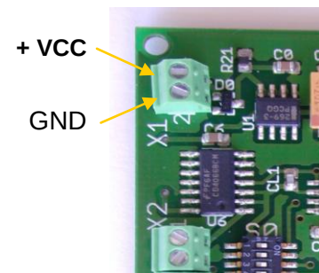
Fig. 2: Power supply connection
