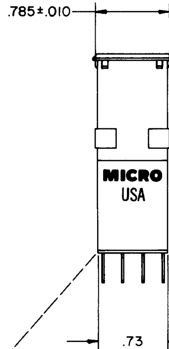
LAMP TERMINAL
